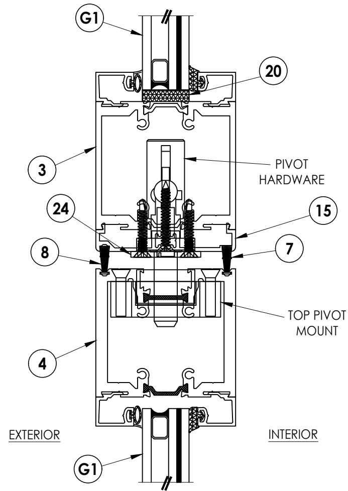
3 4 VERTICAL CROSS SECTION
